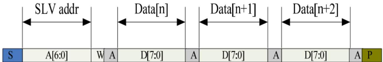
I2C Serial Data Transfer Format
