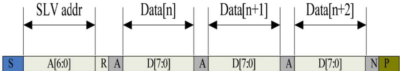
I2C master write, slave read
